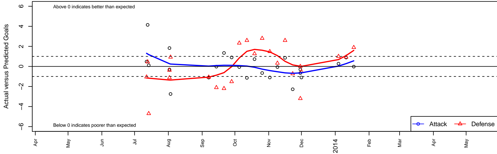
NSC Vortex B01 Dots are actual minus expected GF (blue circles) and GA (red triangles). Blue line is smoothed change in attack strength. Red is smoothed change in defense strength.
